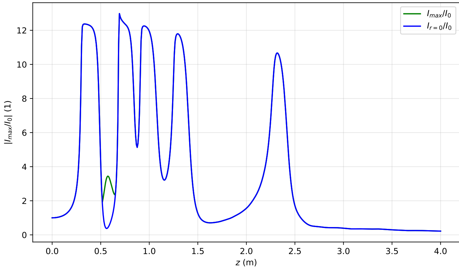
I_{\max}(x = 0, y = 0, z)/I_0 , \text{Pin}=9.0\text{Pcr} , artificial time
